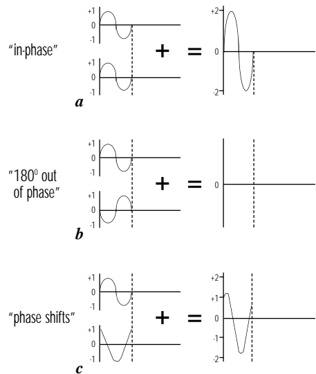
phase relationships
